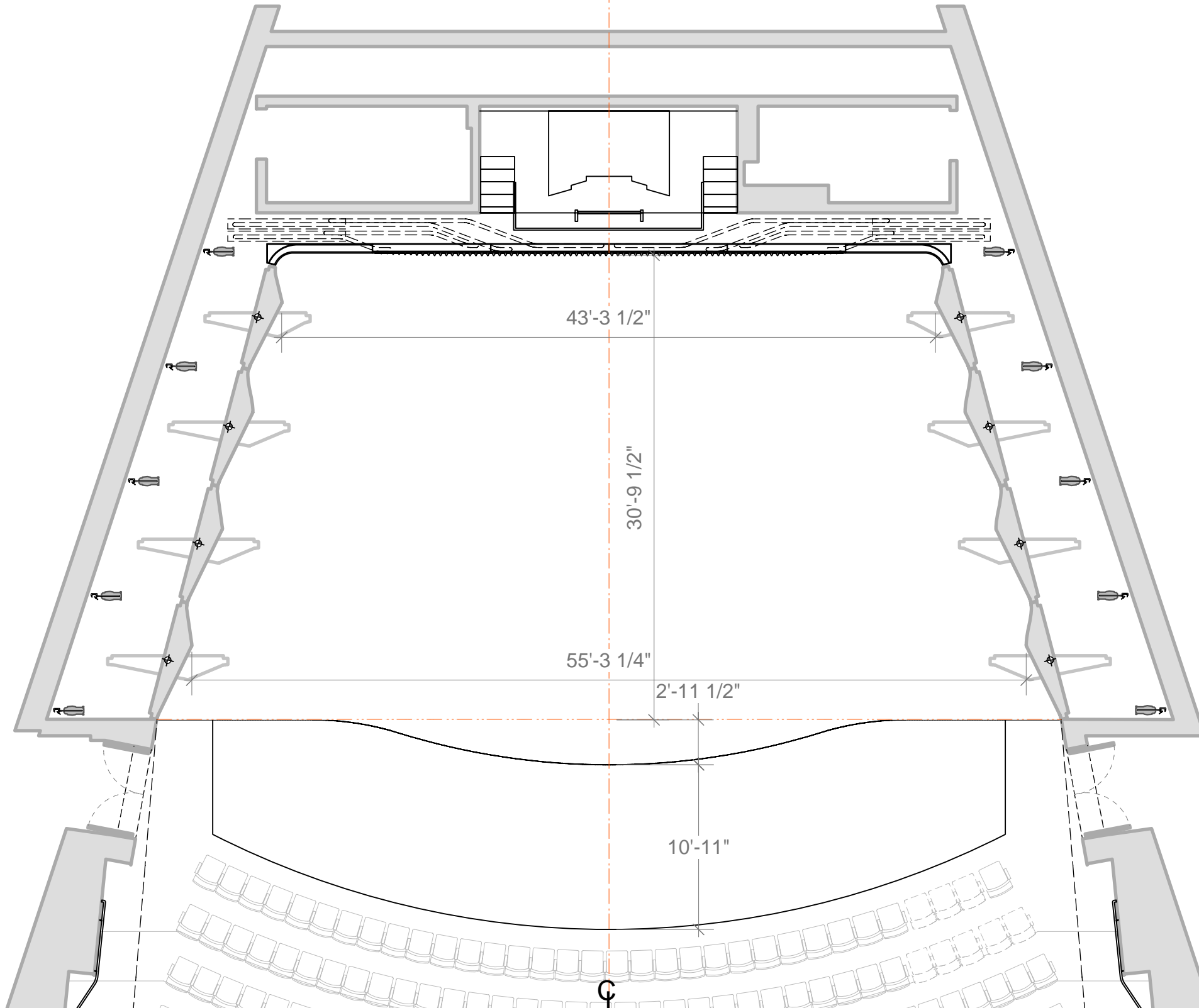
Alice Tully Hall Scale 1/8" = 1'-0"
