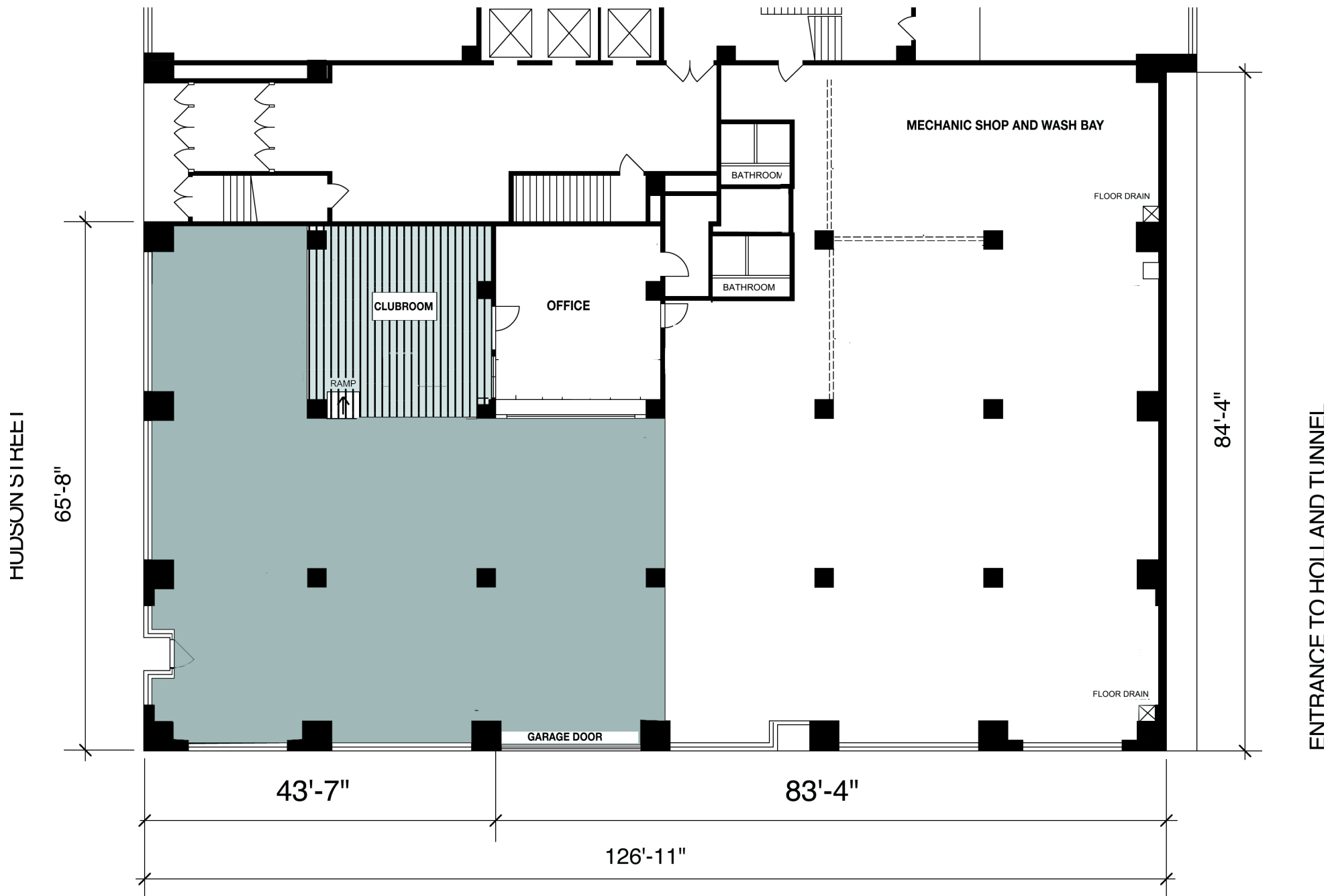
1.2 250 HUDSON STREET: PLAN (ALTERNATE) 1/16" = 1'-0"
